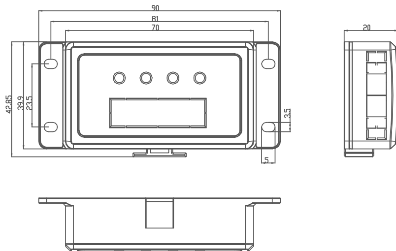
Flex Pixel Driver Dimensional Drawing
